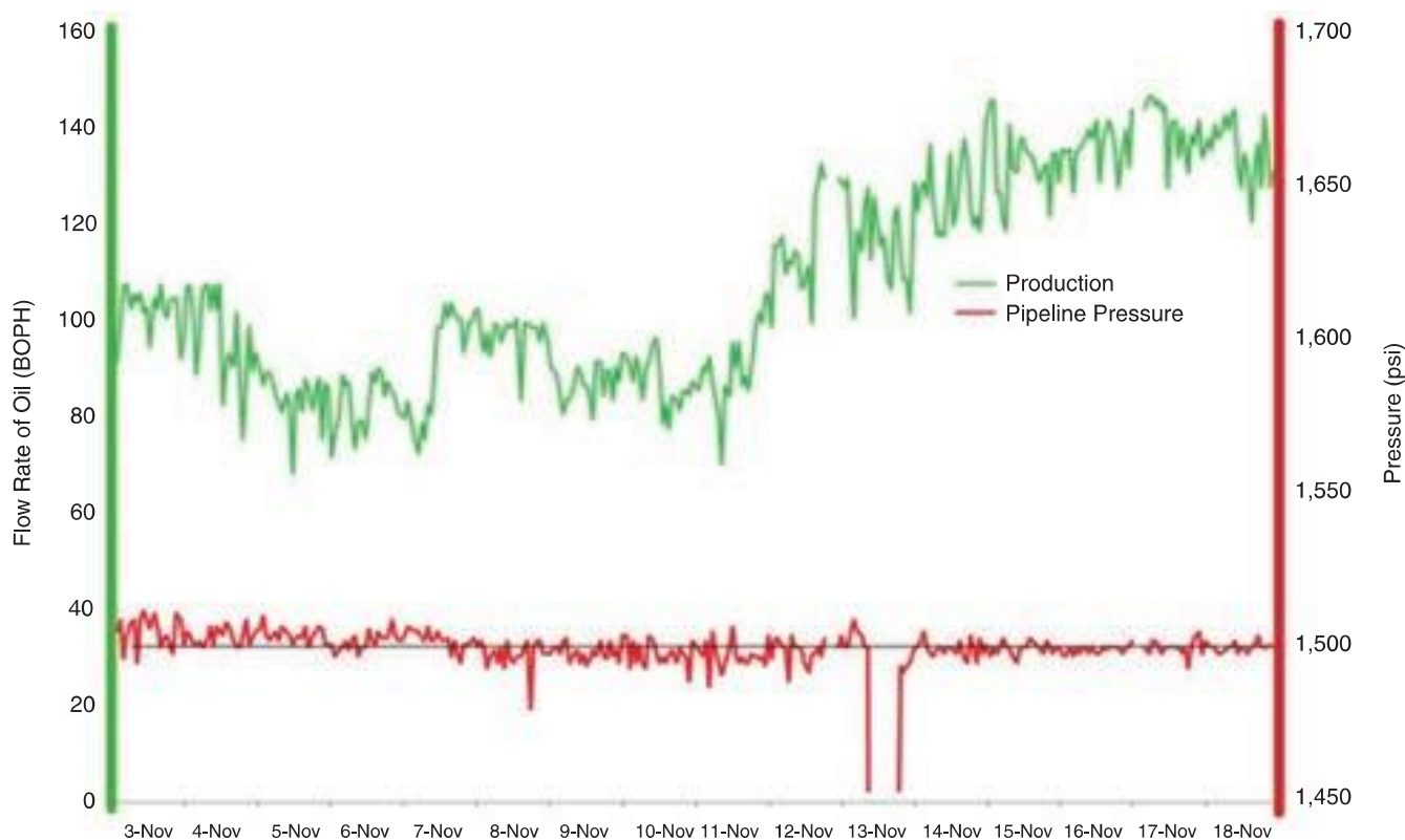
Fig. 2—The improvement in the flow rate of a subsea oil pipeline in the US Gulf of Mexico during wax removal with the Paralax waxophobic nanochemical treatment. Graph courtesy of Diversitech.
